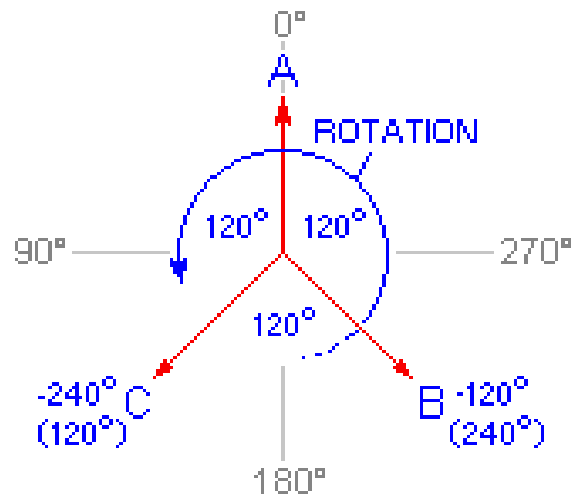
Figure 15. ABC Phase Rotation
