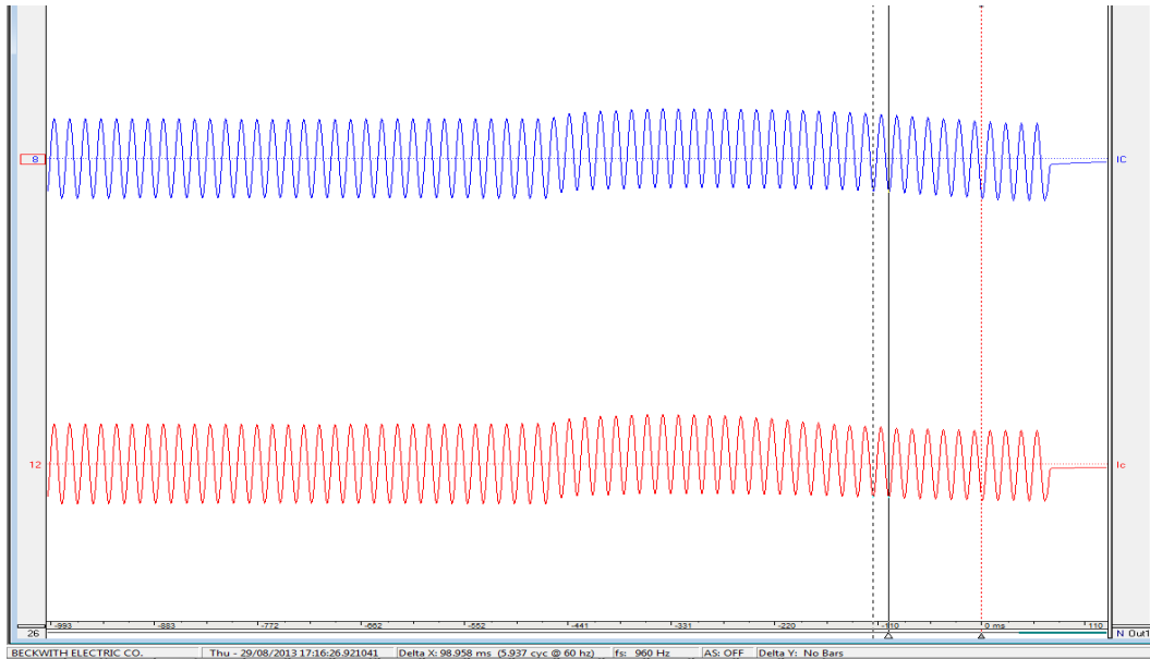
Figure 4A. Generator C-Phase Current
