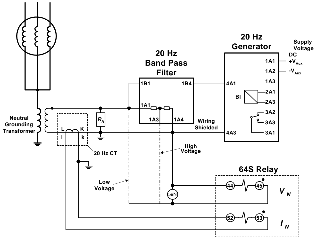
Figure 12. 64S Protection Connection Diagram
