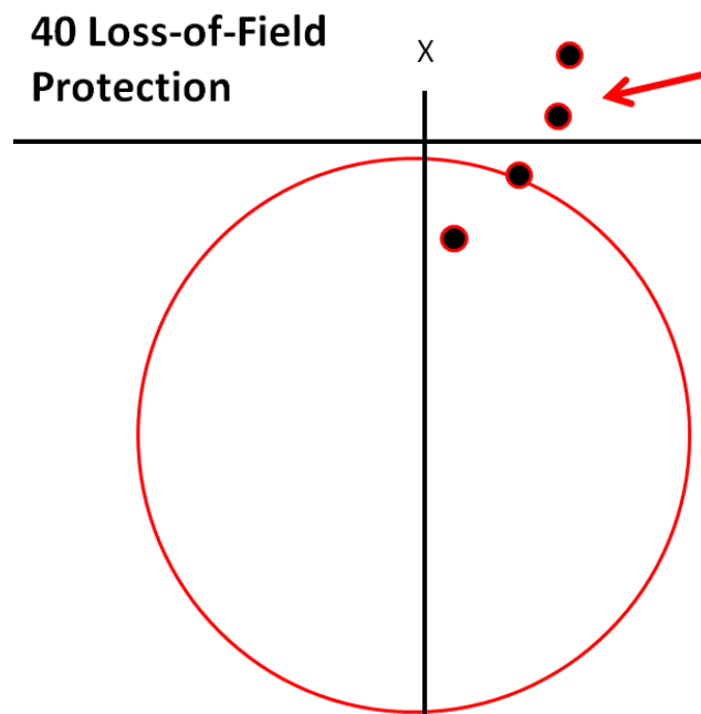
Figure 16. 40 Loss-of-Field Protection
