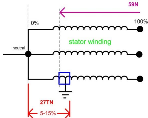
Figure 10. 27TN and 59N Zones of Stator Ground Fault Protection
