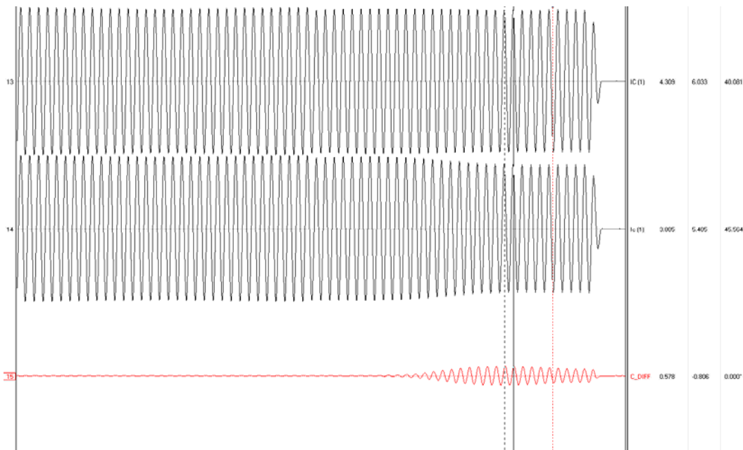
Figure 4B. Generator C-Phase Differential Current
