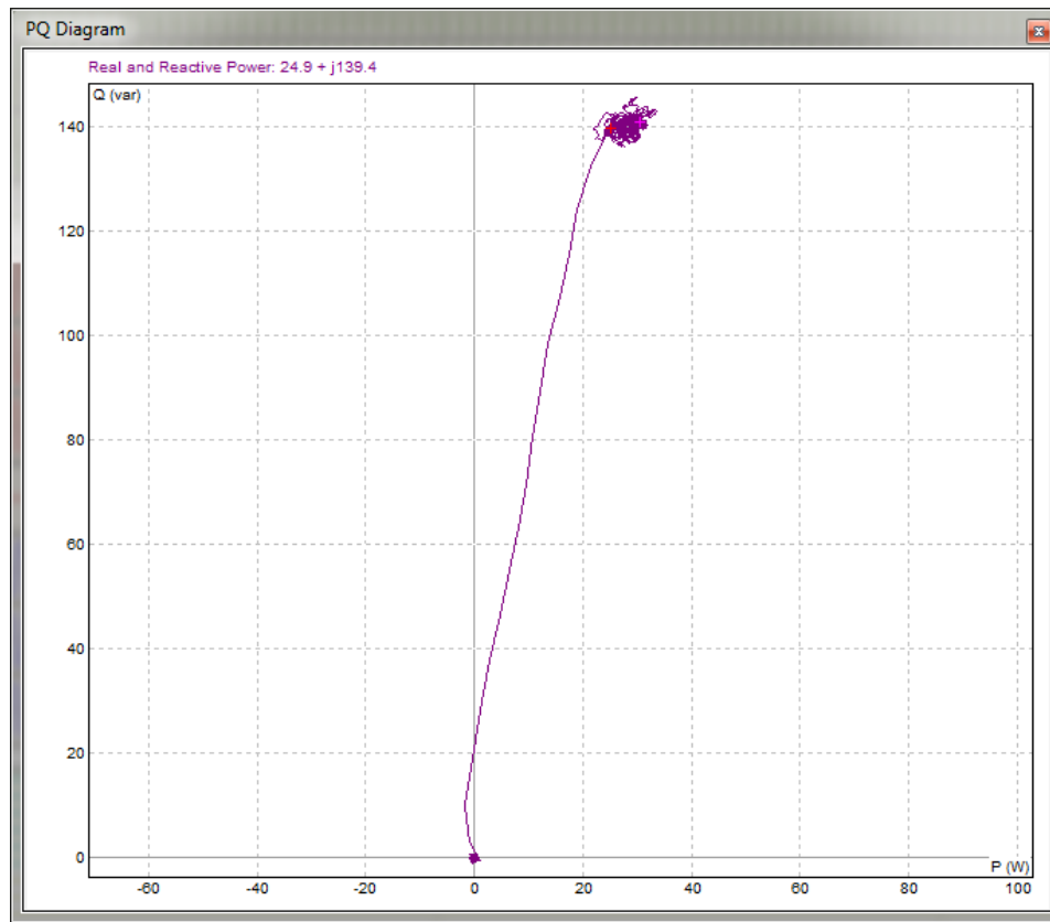
Figure 9. Machine Real and Reactive Power at time of 27TN Trip
