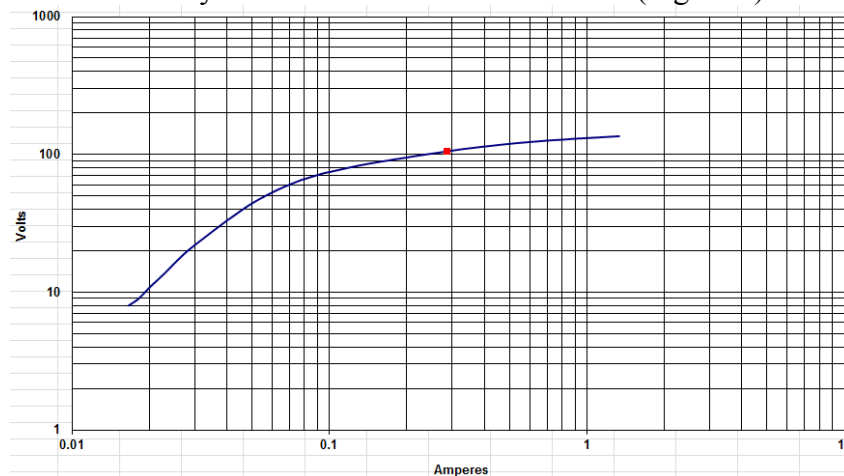
Figure 3. C Phase Neutral Side CT Excitation Characteristic
