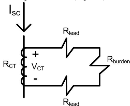
Figure 8. CT Saturation Calculation
