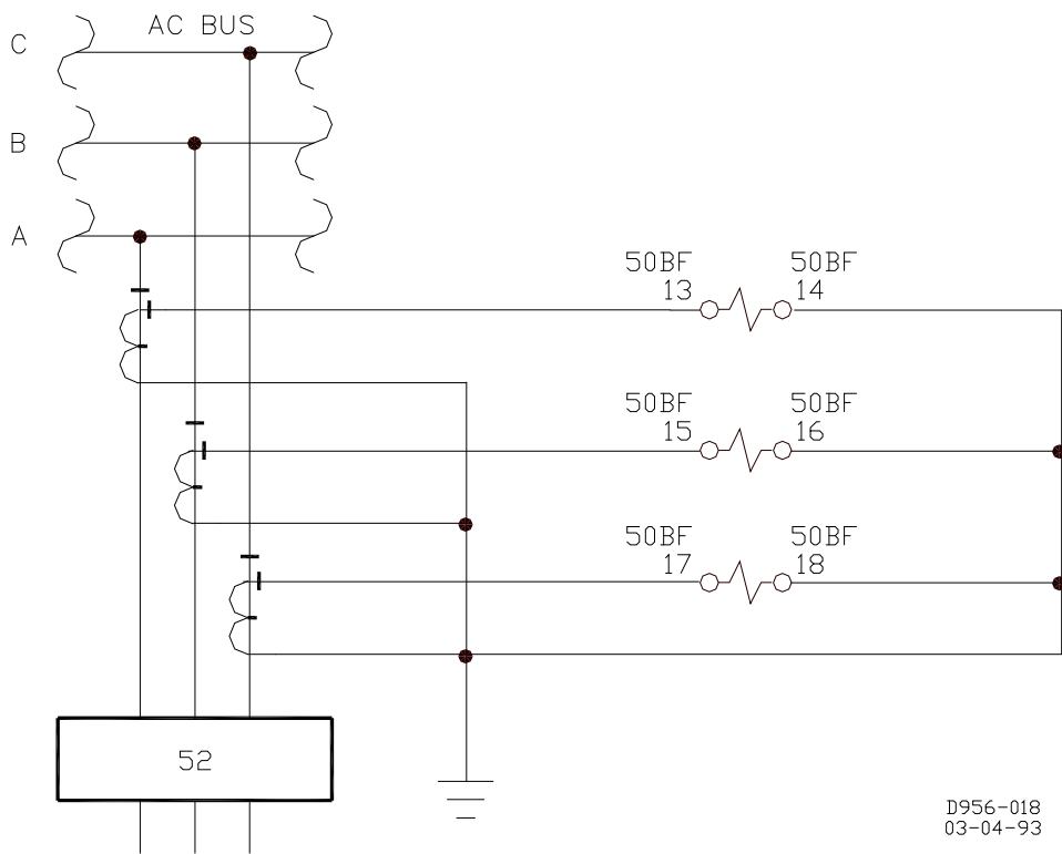
Figure 4-11. Typical Connections Sensing Input Type F
