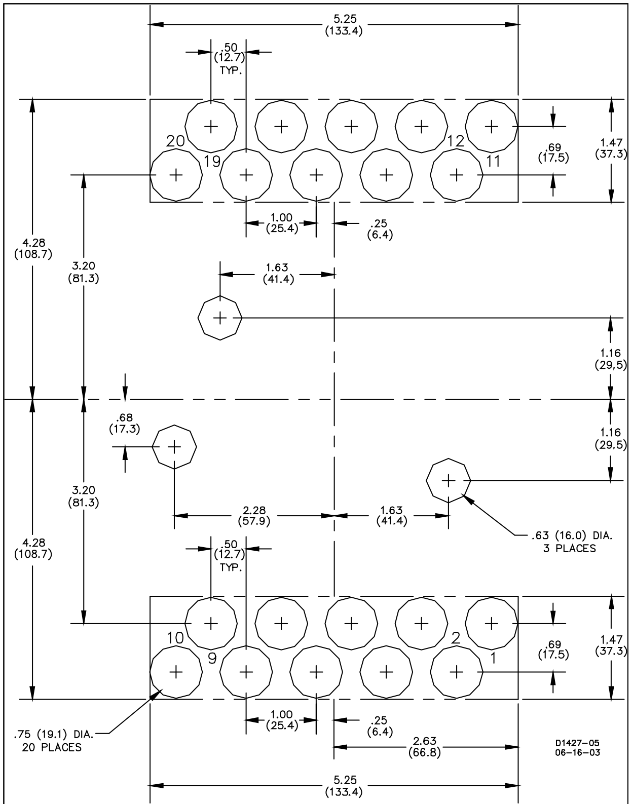
Figure 4-4. Panel Drilling Dimensions, Projection Mounting, Double-Ended Case
