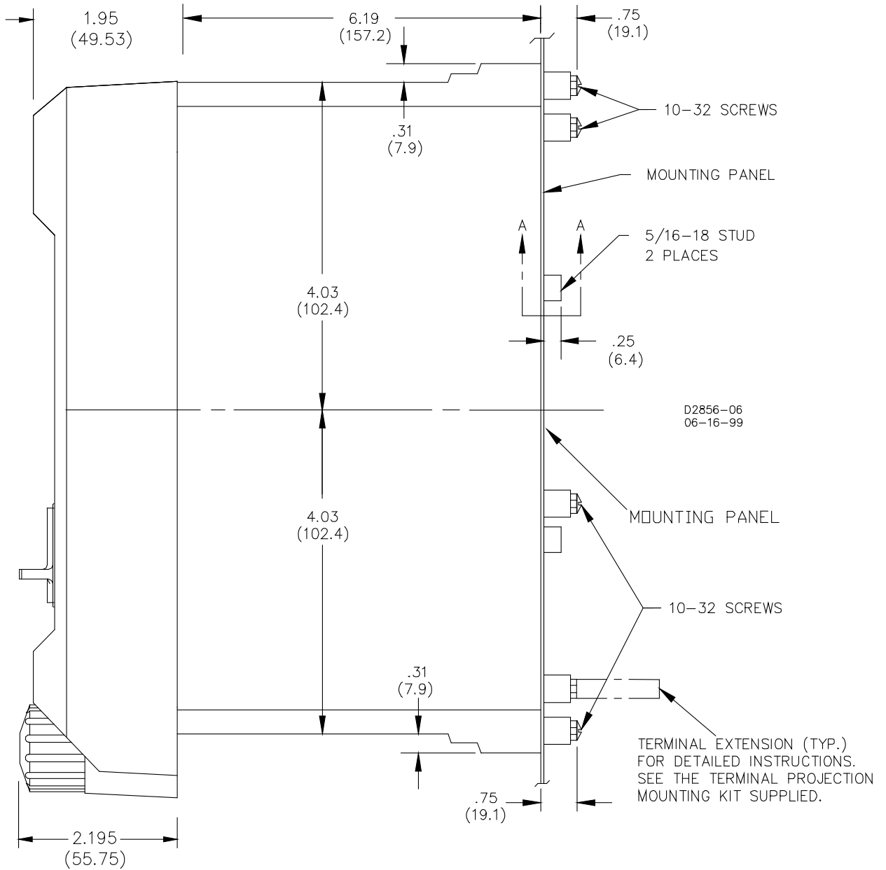
Figure 4-2. Outline Dimensions, Side View, Projection Mounted, Double-Ended Case
