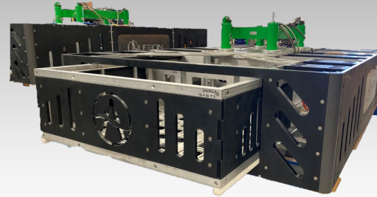
Multiple ROV Skid Configurations
