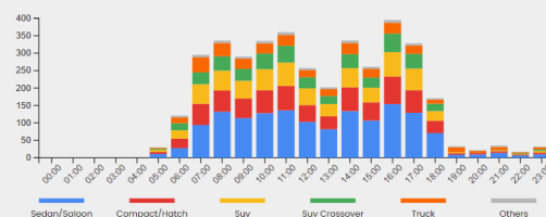
Average Body Types Per Hour
