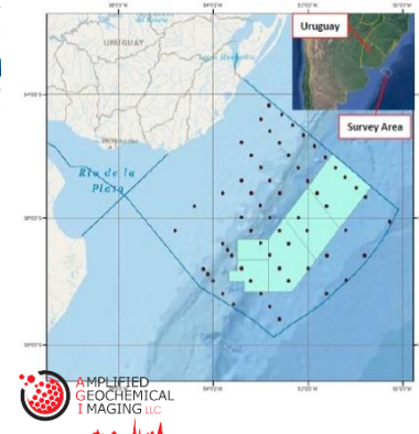
AGI: micro-seeps detection of hydrocarbons into sediment samples
