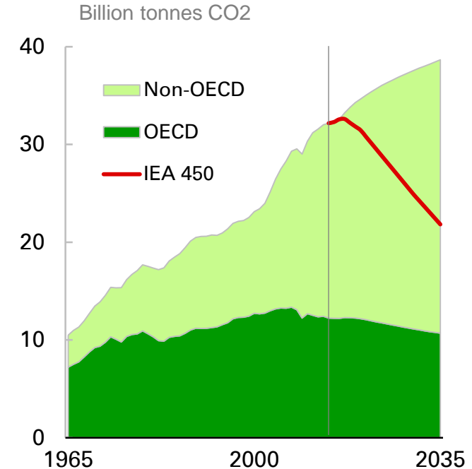
Carbon emissions
